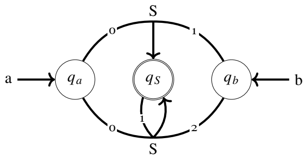
Figure 7.4: S \rightarrow aSb and S \rightarrow ab as a labeled ordered directed hypergraph. Each rule is represented by a hyperedge, and accepting states are represented by being doubly outlined.
