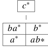
Figure 4.13: A language in \mathbb{D}\mathbf{A} but not \mathbb{L}\mathbf{L} , proving incomparability
