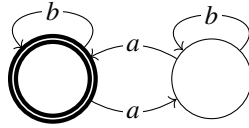
Figure 2.4: A finite-state string acceptor: doubly-outlined states are accepting, and the initial state is marked by the thick outline. All and only those strings which contain an even number of occurrences of a are accepted.
