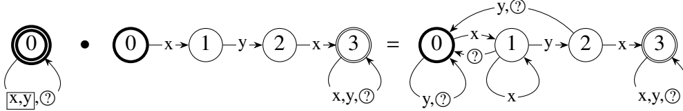
Figure 3.8: Canonical AAA for the free factor “xyx” under \triangleleft constructed via concatenation. The boxed \boxed{x,y} in the first operand are symbols that needed to be added for compatibility.
