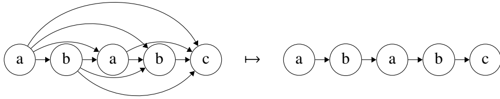
Figure 2.1: Precedence and successor models of “ababc”.
