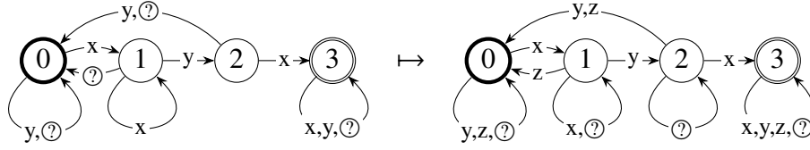
Figure 3.9: Relativizing “xyx” to T = \{x, y, z\} : Add ‘z’ in parallel to any existing \textcircled{?} edges, remove those \textcircled{?} edges, then add new \textcircled{?} edges as self-loops everywhere.
