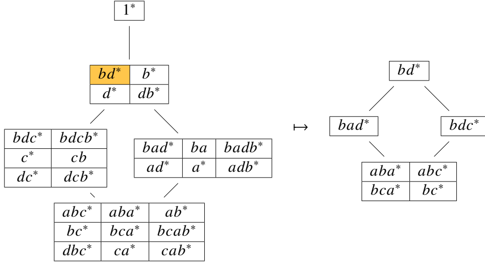
Figure 4.11: Egg-box for “contains a not preceding bc and c not following ab ”.
