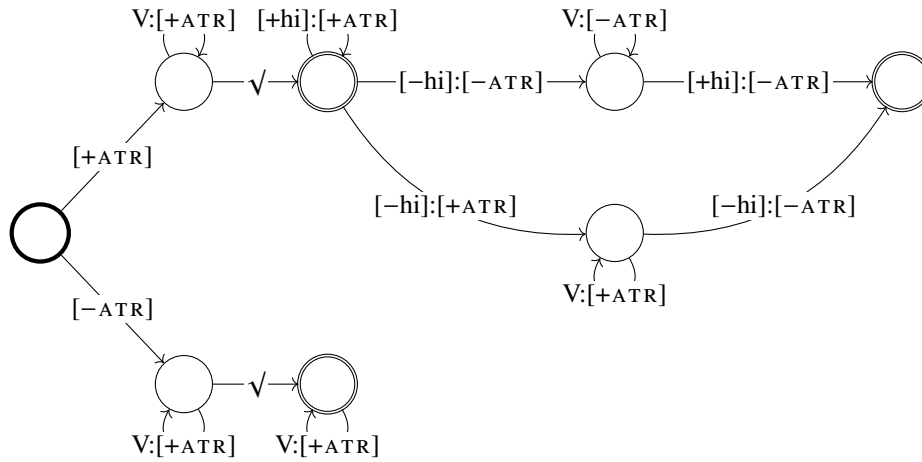
Figure 5.16: Nondeterministic transducer for Tutrugbu ATR harmony.
