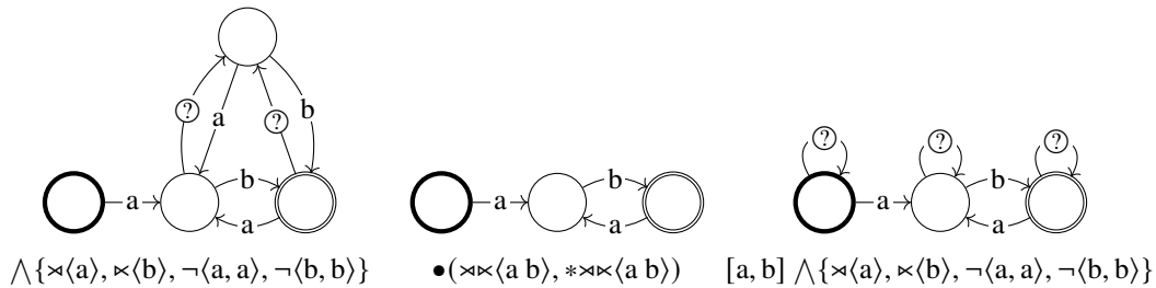
Figure 9.1: Three definitions for one language over \Sigma = \{a, b\} , and semantics.
