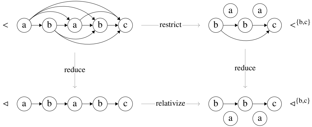
Figure 3.2: Word models for “ababc” using general precedence, immediate successor, and relativized variants of each, showing the relationships among these relations. Domain elements that are not ordered are pulled aside from the structure. In these examples, the alphabet is \Sigma = \{a, b, c\} , and the salient symbols for the relativized relations are T = \{b, c\}
