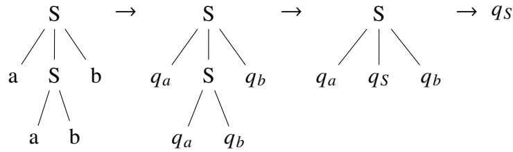
Figure 7.1: Accepting a tree.
