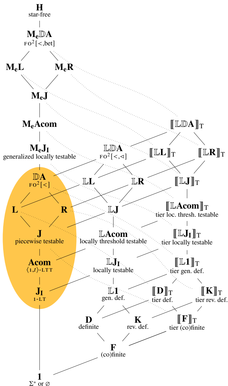
Figure 4.16: The full algebraic hierarchy. It is essentially a crystal formed by copies of the highlighted region, but the lower levels are degenerate. Some lines dotted for readability.
