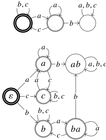
Figure 5.1: The acceptors induced by Nerode (above) and Myhill (below) equivalence for a string language forbidding ab substrings.
