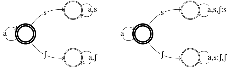
Figure 5.8: Samala sibilant harmony: \mathbb{N} -minimal trimmed acceptor (left) and \mathbb{M} -minimal transducer (right). Outputs omitted when identical to inputs.
