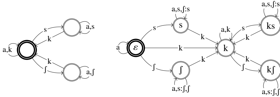
Figure 5.9: A variant of Samala sibilant harmony, adding blockers: \mathcal{N} -minimal trimmed acceptor (left) and \mathcal{M} -minimal transducer (right).
