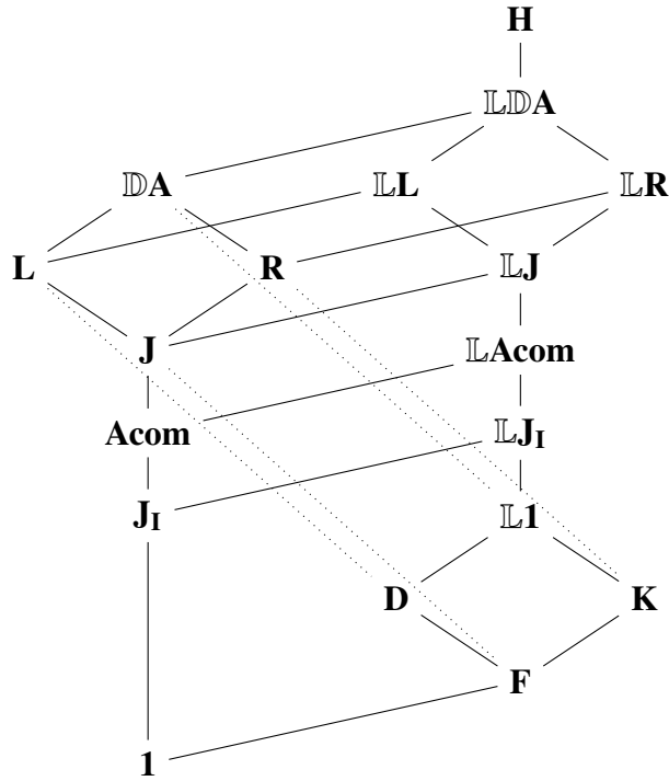
Figure 4.15: The hierarchy including sub- \mathbb{L}1 classes and M_e -based connections.
