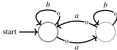
Figure 7.8: The string acceptor of Figure 7.2 as an ordered directed hypergraph. The two are identical, except that this version has additional labels for the sequence indices, which are always zero.
