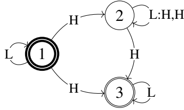
Figure 5.11: High-tone plateauing as a one-way nondeterministic machine.
