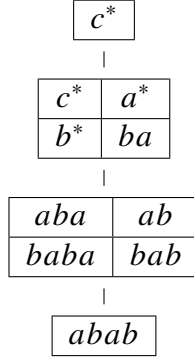
Figure 4.14: A language in \mathbb{L}\mathbf{Acom} but not \mathbb{L}\mathbf{J_1} or \mathbb{D}\mathbf{A} .
