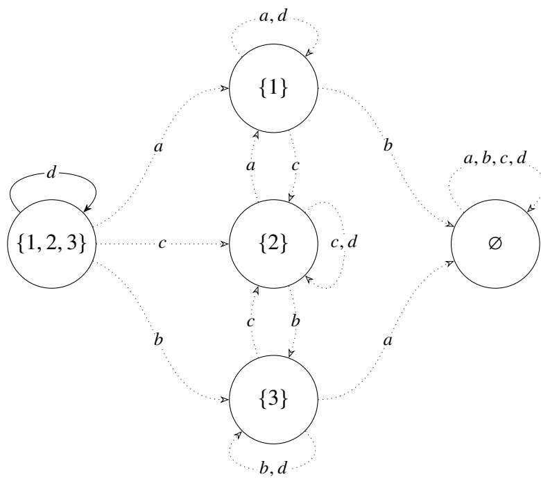
Figure 3.5: The powerset graph that corresponds to the DFA of Figure 3.4, with the cycle marked that proves this stringset is not SL. Notice that if d is removed, there is no such cycle.
