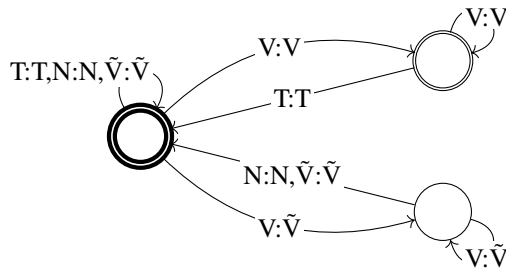
Figure 5.5: Nondeterministic transducer for oppositeward nasal spreading.
