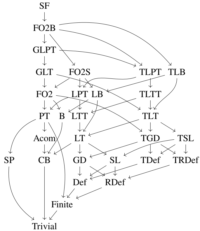
Figure 9.2: Hierarchy of classes for which decision algorithms are provided.
