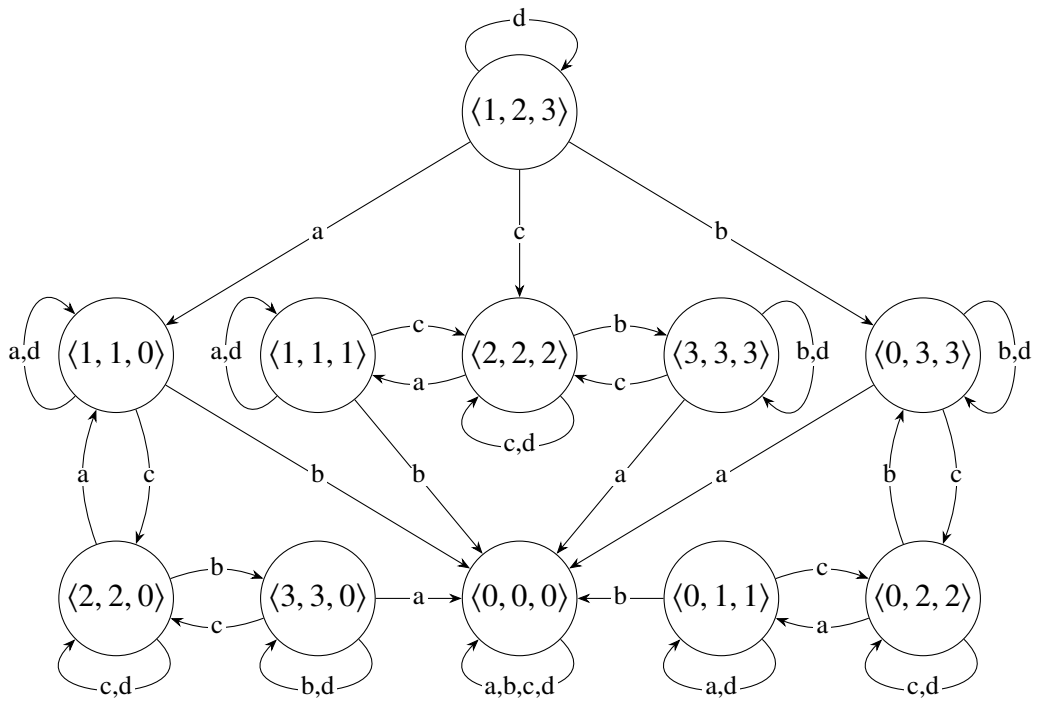
Figure 3.10: The syntactic semigroup corresponding to the DFA of Figure 3.4. Each function is represented by the image of \langle 1, 2, 3 \rangle . (Each tuple additionally has a fourth entry that is always labeled 0 and is omitted here for brevity.) The corresponding projected subsemigroup lacks the identity as well as every edge labeled d .
