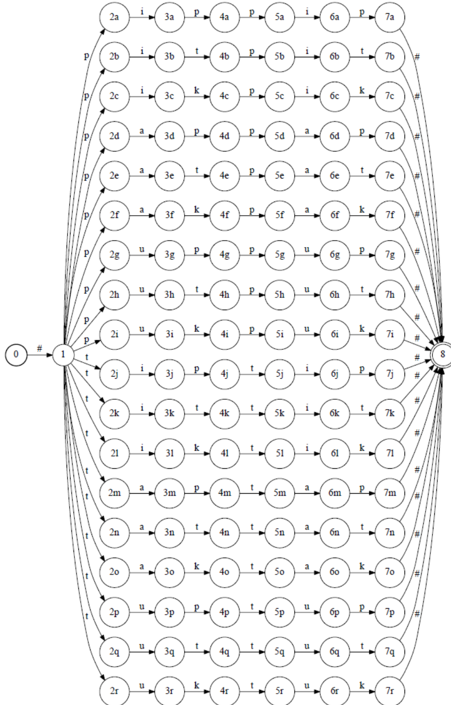
(15) A finite-state acceptor for Balinese pseudoreuplicated stems (6-phoneme inventory)
